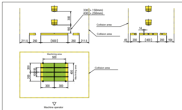
Speedio S500X1
